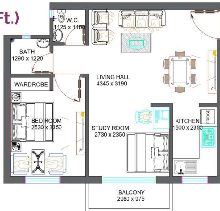
1 BHK + Study(505 Sq.Ft.)
